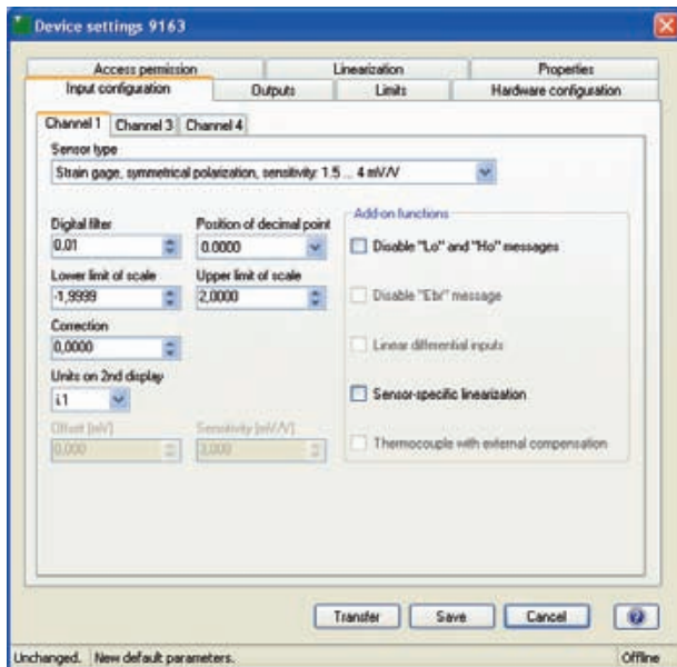
Instrument parameterization
